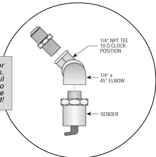
Fig. 2-b / Driver's Side View
